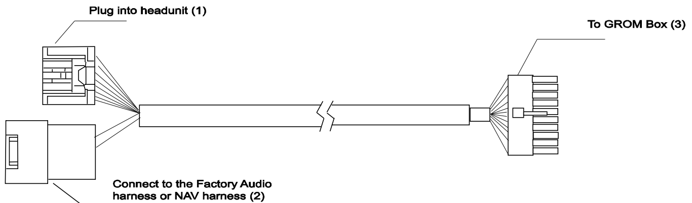
Figure 4. Connection scheme for Toyota/Lexus/Scion and Honda/Acura
