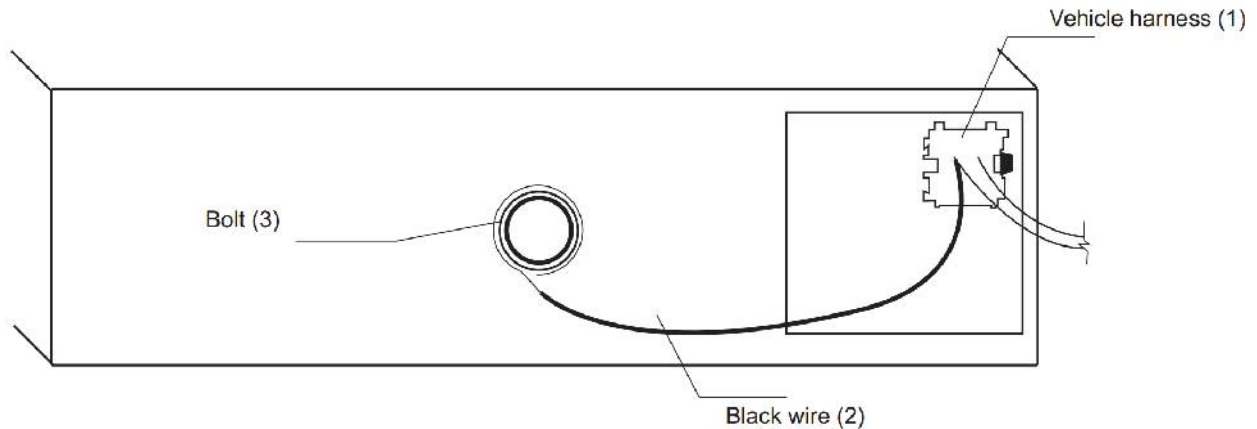
Figure 3. Wire grounding for VW/AUDI Installs
